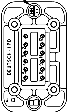
DT15-12PB COLOR BLACK
