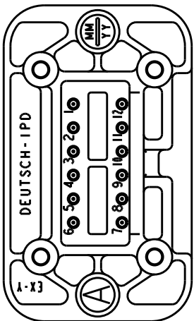
DT15-12PA COLOR GREY
