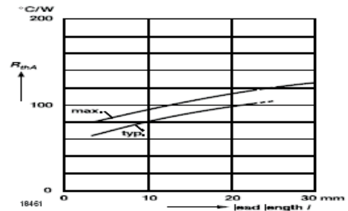
FIG.4- THERMAL RESISTANCE VS LEAD LENGTH
