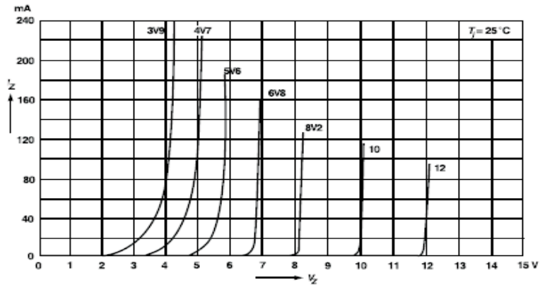
FIG.7- BREAKDOWN CHARACTERISTICS
