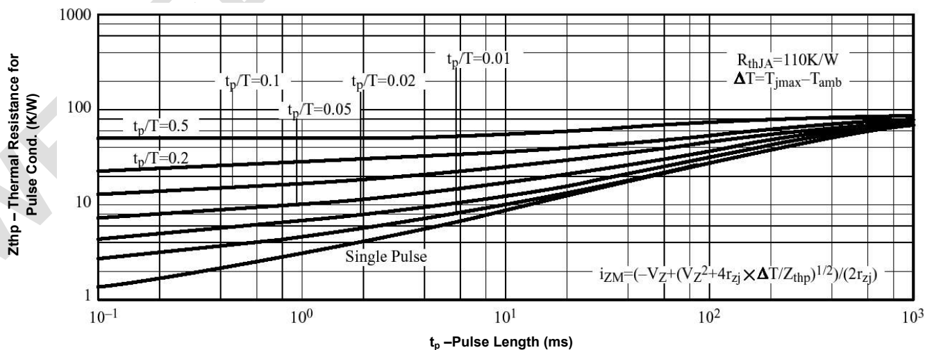
Figure5. Thermal Response
