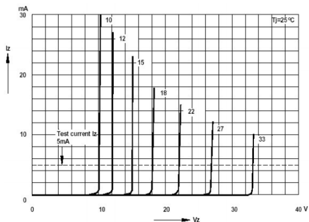
Fig.2- Breakdown characteristics
