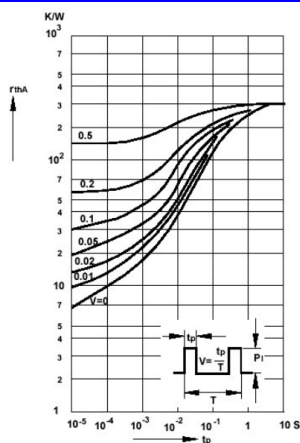
Fig.5-Pulse thermal resistance versus pulse duration
