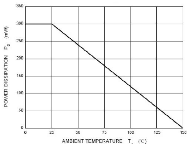
Fig.4- Admissible power dissipation versus ambient temperature
