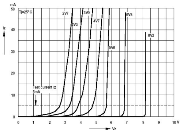
Fig.1-Breakdown characteristics
