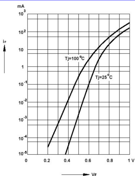
Fig.3- Forward characteristics
