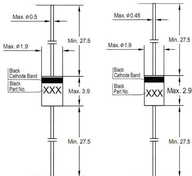
Glass Case DO-35 Dimensions in mm
