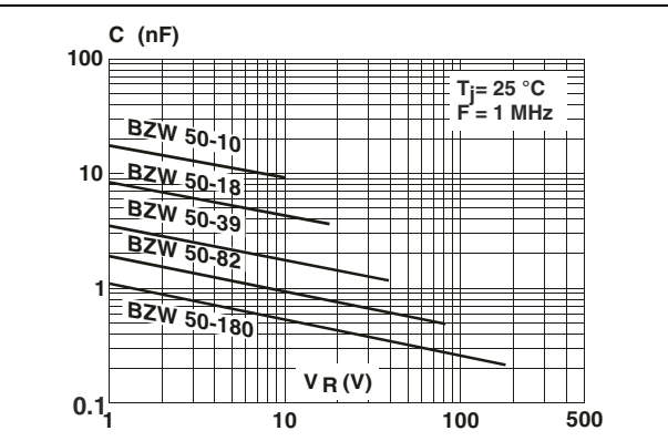
Figure 6. Capacitance vs. reverse applied voltage for unidirectional types (typical values).
