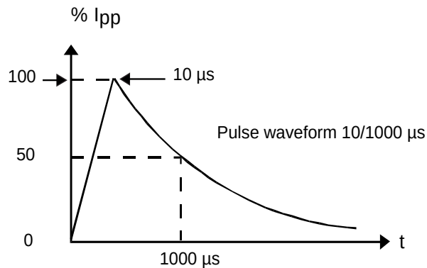
Figure 2: Pulse waveform (10/1000 \mu s)
