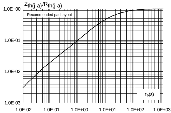
Figure 9: Relative variation of thermal impedance junction to ambient versus pulse duration (printed circuit board FR4, e_{CU} = 35 \text{ }\mu\text{m} )
