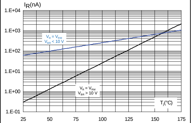
Figure 10: Leakage current versus junction temperature
