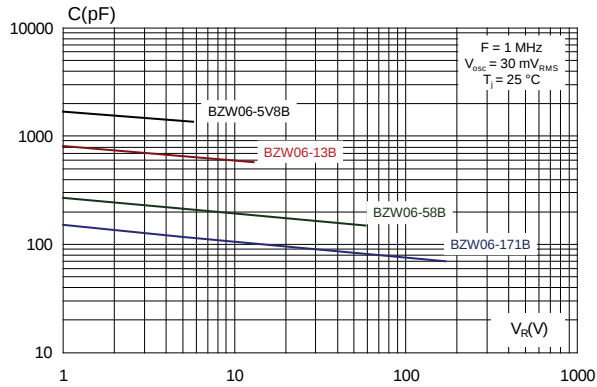
Figure 7: Junction capacitance versus reverse applied voltage (bidirectional types)
