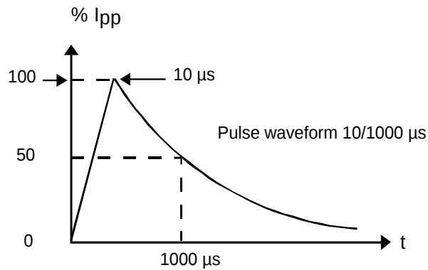
Figure 2: Pulse waveform (10/1000 \mu s)
