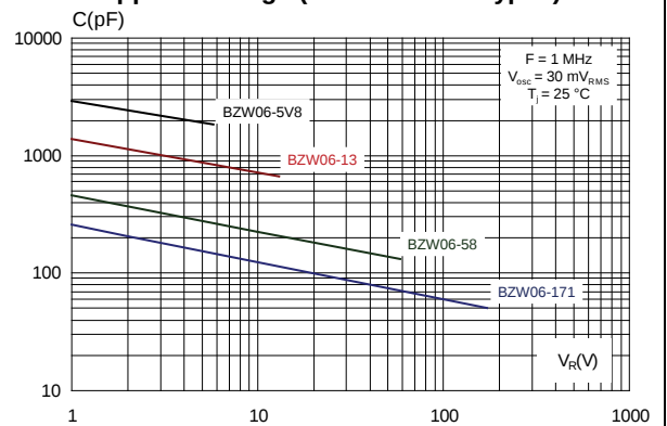
Figure 6: Junction capacitance versus reverse applied voltage (unidirectional types)
