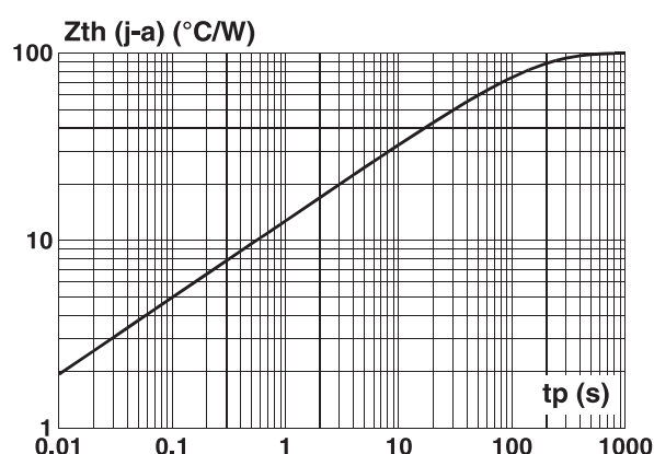
Fig. 3: Transient thermal impedance junction ambient versus pulse duration (For FR4 PC Board with L lead = 10mm).
