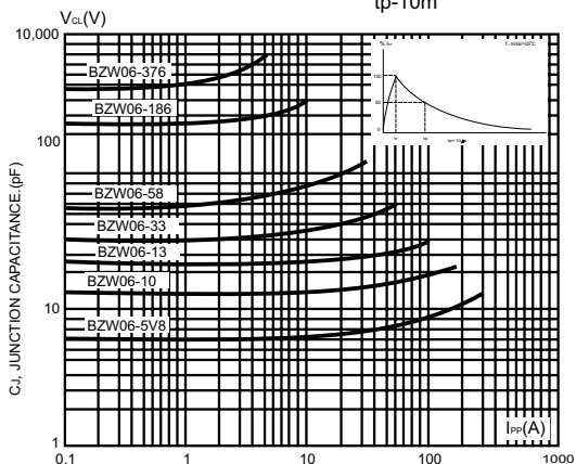
FIG.4- CLAMPING VOLTAGE VERSUS PEAK PULSE CURRENT. EXPONENTIAL WAVEFORM tp=200μs tp=1ms tp=10m
