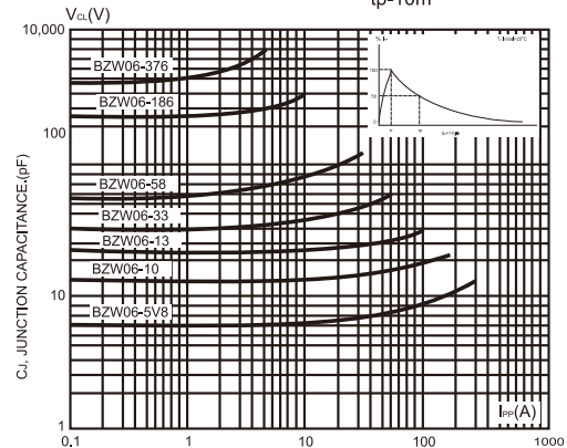
FIG.4- CLAMPING VOLTAGE VERSUS PEAK PULSE CURRENT. EXponential WAVEFORM tp=200µs tp=1ms tp=10m
