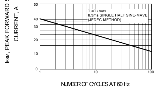
FIG.6 – MAXIMUM NON-REPETITIVE FORWARD SURGE CURRENT UNIDIRECTIONAL ONLY
