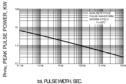
FIG.3 – PULSE WAVEFORM
