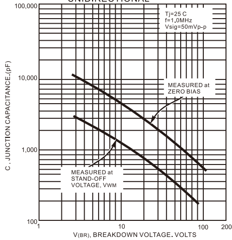
FIG.7- TYPICAL JUNCTION CAPACITANCE UNIDIRECTIONAL
