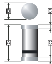
SOD-80 (Mini-MELF)
