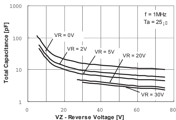
Figure 2. Total Capacitance
