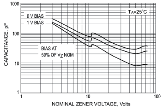
Fig.4 TYPICAL CAPACITANCE
