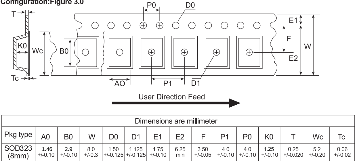
SOD323 Embossed Carrier Tape Configuration:Figure 3.0
