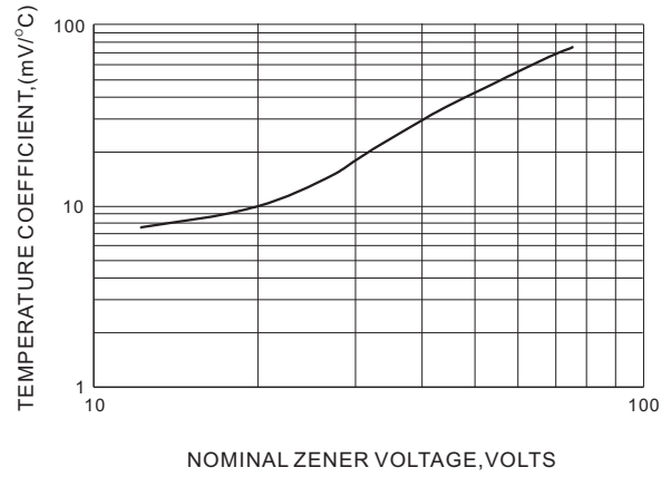
Fig.2 TEMPERATURE COEFFICIENTS
