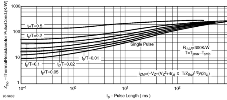
Fig. 13 Thermal Response
