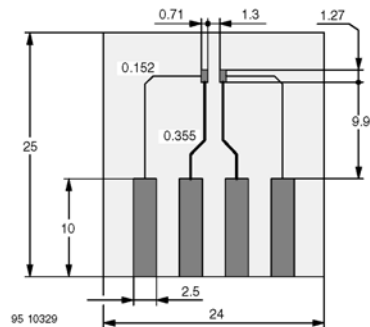
Fig. 10 Board for R_{thJA} definition (in mm)
