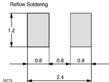
Fig. 11 Recommended foot pads (in mm)
