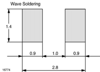
Fig. 12 Recommended foot pads (in mm)
