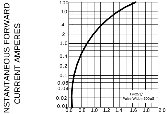
FIG.2 –TYPICAL FORWARD CHARACTERISTIC
