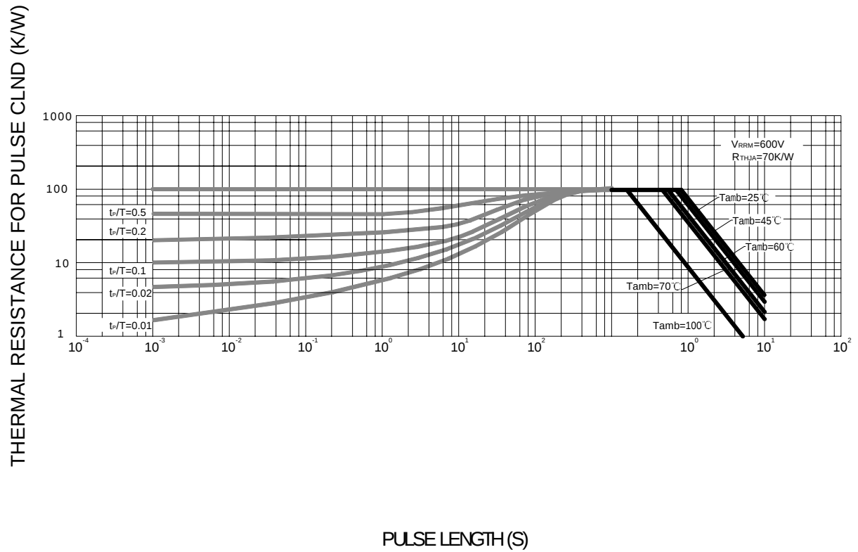
FIG.8 -THERMAL RESPONSE
