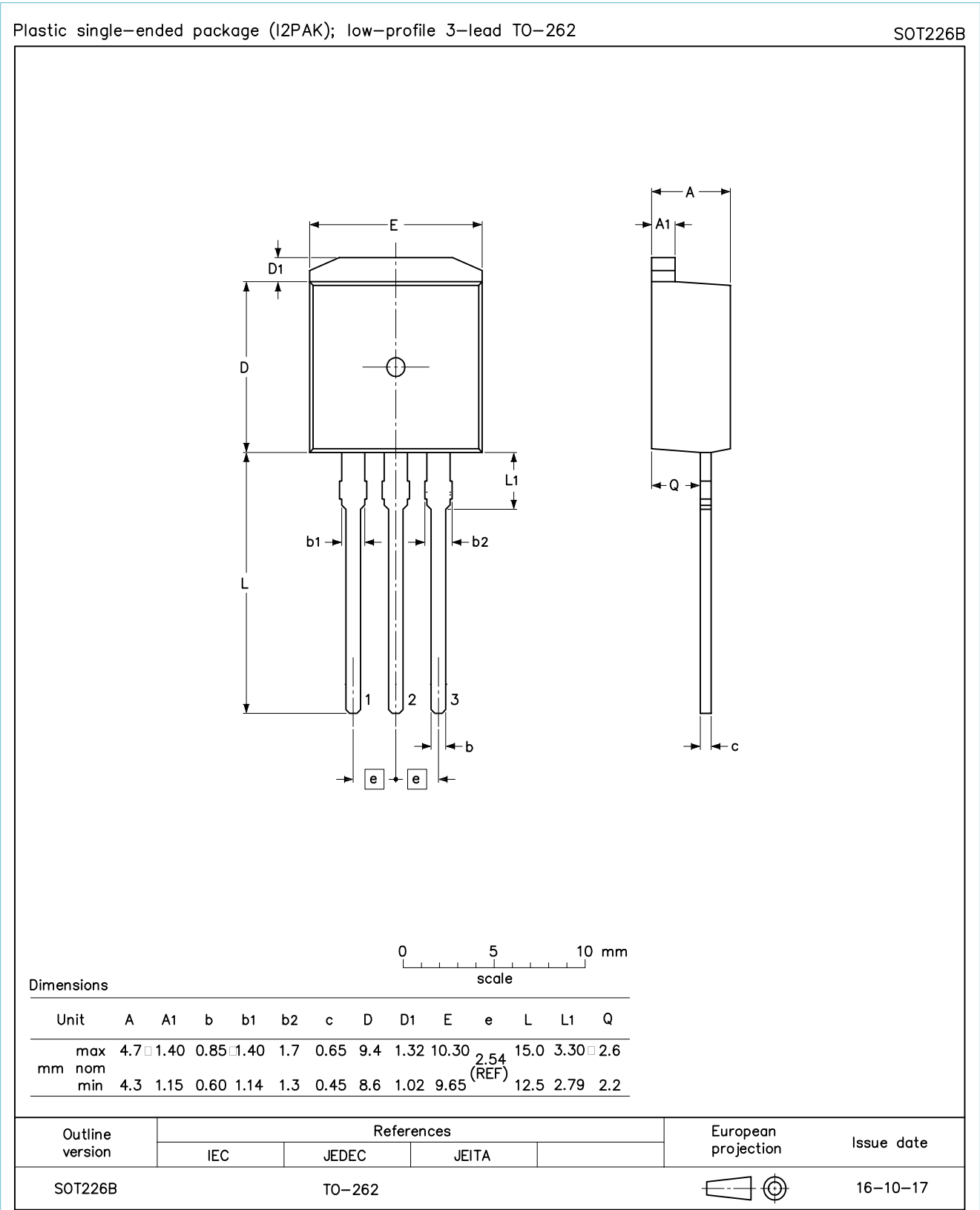
Fig. 1. Package outline I2PAK (SOT226B)
