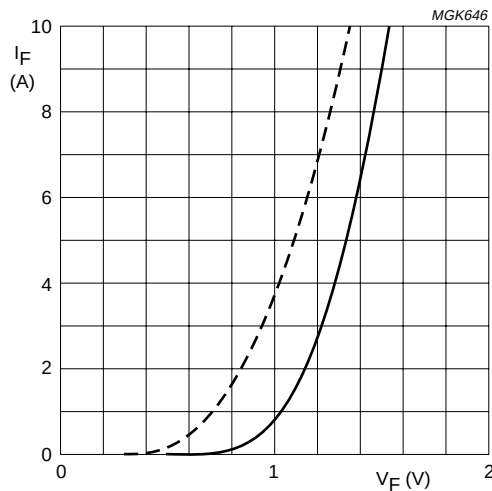
BYV28-500 and 600 Dotted line: T_j = 175^\circ\text{C} . Solid line: T_j = 25^\circ\text{C} .
