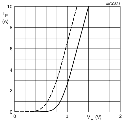
BYV28-300 and 400 Dotted line: T_j = 175^\circ\text{C} . Solid line: T_j = 25^\circ\text{C} .
