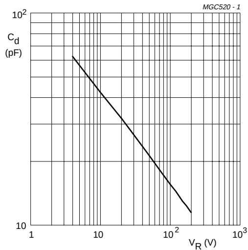
BYV28-300 and 400 f = 1\text{ MHz} ; T_j = 25\text{ }^\circ\text{C} .
