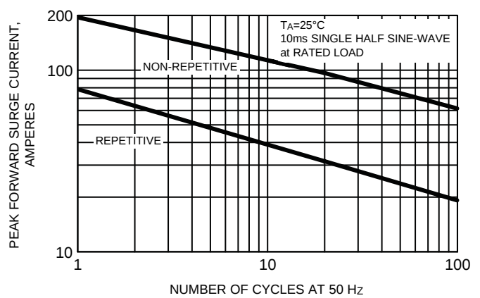
FIG. 2 - MAXIMUM PEAK FORWARD SURGE CURRENT
