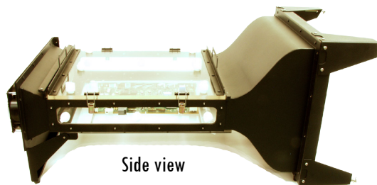
WTC-100™ Wind Tunnel Controller
