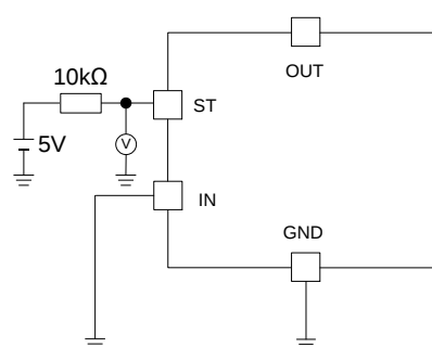
Measurement Circuit for Figure 24
