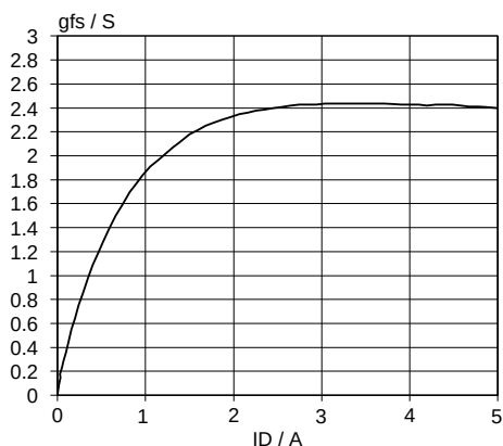
Fig. 8. Typical transconductance, T_j = 25^\circ \text{C} . g_{fs} = f(I_D) ; conditions: V_{DS} = 25 \text{ V}
