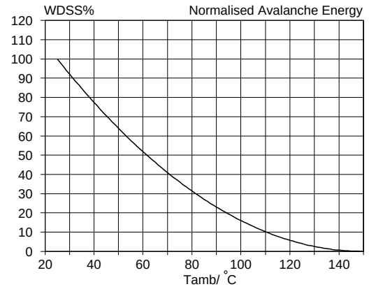
Fig.15. Normalised avalanche energy rating. W_{DSS}\% = f(T_{amb}) ; conditions: I_D = 0.9 \text{ A}
