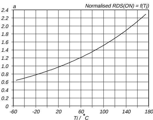
Fig.9. Normalised drain-source on-state resistance. a = R_{DS(ON)}/R_{DS(ON)25\text{ °C}} = f(T_j) ; I_D = 13 A; V_{GS} = 5 V
