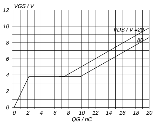
Fig.13. Typical turn-on gate-charge characteristics. V_{GS} = f(Q_G) ; conditions: I_D = 13\text{ A} ; parameter V_{DS}
