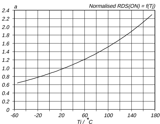
Fig.9. Normalised drain-source on-state resistance. a = R_{DS(ON)}/R_{DS(ON)25\text{ °C}} = f(T_j) ; I_D = 6.5 A; V_{GS} = 5 V
