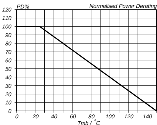
Fig.1. Normalised power derating. PD\% = 100 \cdot P_D / P_{D\ 25\ ^\circ C} = f(T_{mb})
