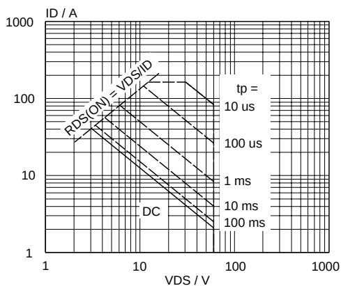
Fig.3. Safe operating area. T_{mb} = 25\ ^\circ C I_D & I_{DM} = f(V_{DS}); I_{DM} single pulse; parameter t_p
