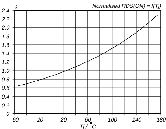
Fig. 9. Normalised drain-source on-state resistance. a = R_{DS(ON)}/R_{DS(ON)25 \text{ }^\circ\text{C}} = f(T_j) ; I_D = 5 \text{ A} ; V_{GS} = 10 \text{ V}
