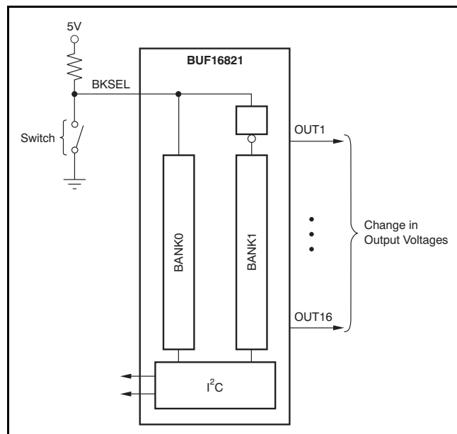
Figure 17. Gamma Control
