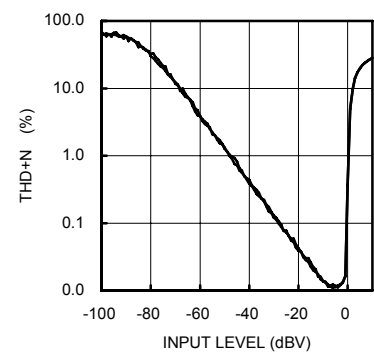
Fig.20 16bit D/A Converter Total Harmonic Distortion (SPOL)
