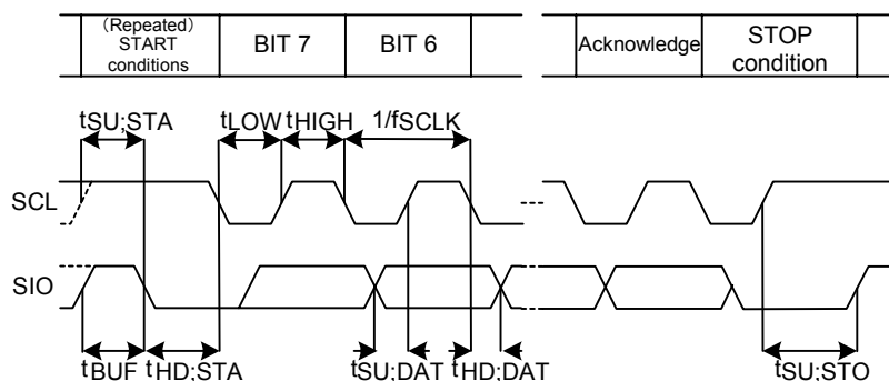
Fig.35 I²C Timing Diagram
