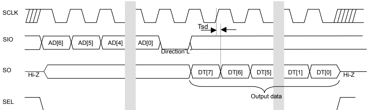
Fig.34 CPU I/F Timing Chart (BU7893GU)
