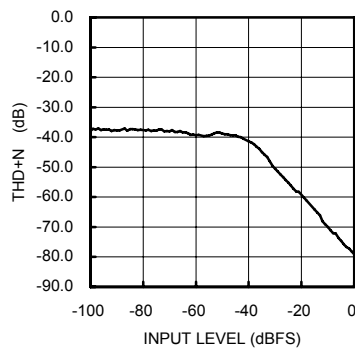
Fig.18 16bit D/A Converter Total Harmonic Distortion 1kHz (SPOL)
