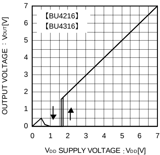
Fig.6 I/O Characteristics
