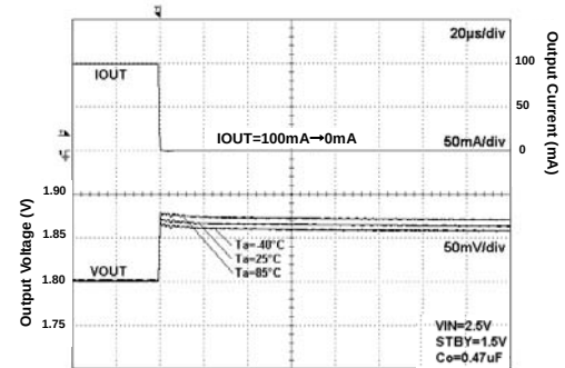
Fig 17. Load Response
