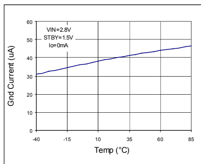
Fig 12. IGND - Temp
