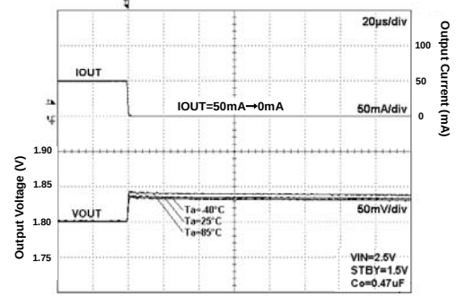
Fig 15. Load Response
