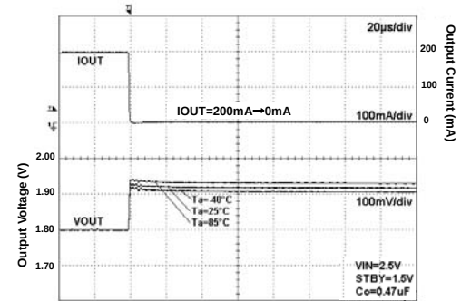
Fig 19. Load Response
