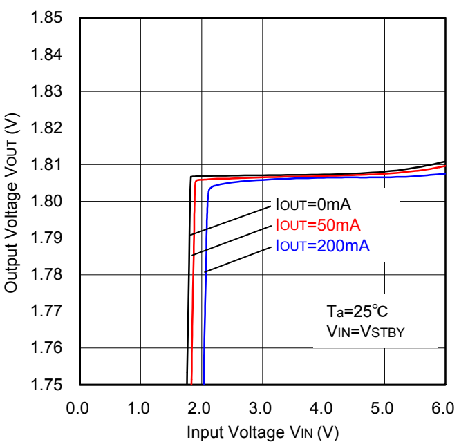
Figure 4. Line Regulation
