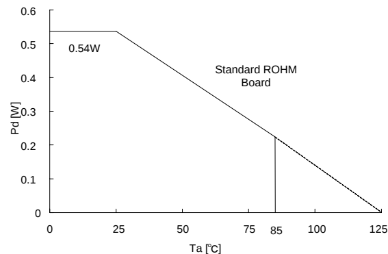
Fig. 23 SSOP5 Power dissipation heat reduction characteristics (Reference)
