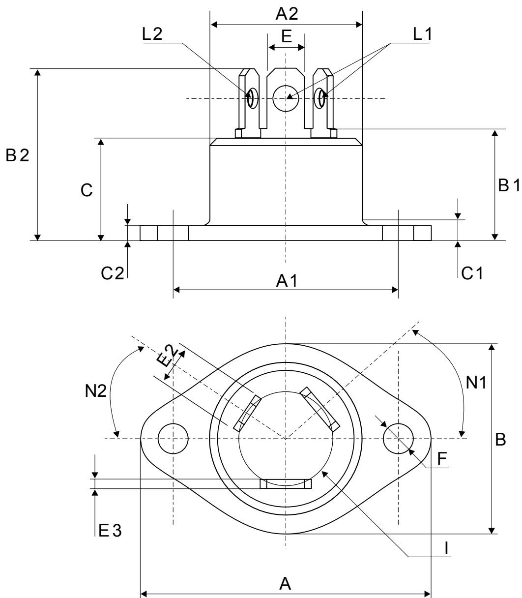
Figure 8. RD91 package outline
