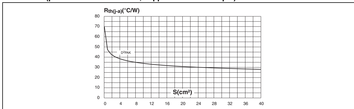
Figure 11. D 2 PAK thermal resistance junction to ambient versus copper surface under tab (printed circuit board FR4, copper thickness: 35 μm)
