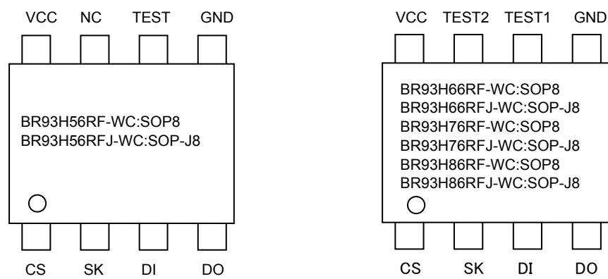
Fig.28 Pin assignment diagram
