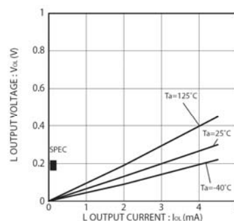
Fig.4 L output voltage V_{OL} -IOL ( V_{CC}=2.7\text{V} )
