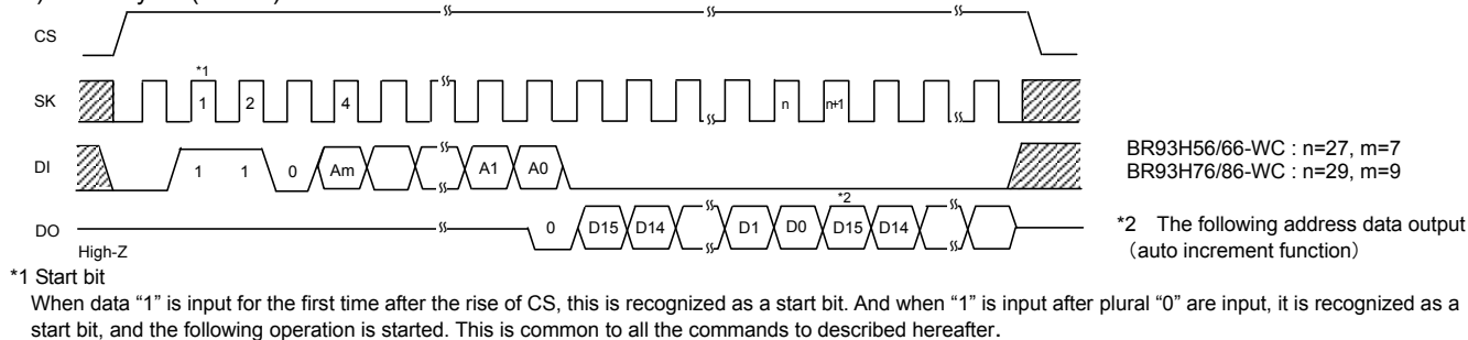
Fig. 30 Read cycle
