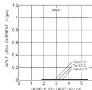
Fig.10 Input leak current I_{LI} (CS,SK,DI)
