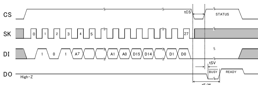
Figure 31. Write Cycle
