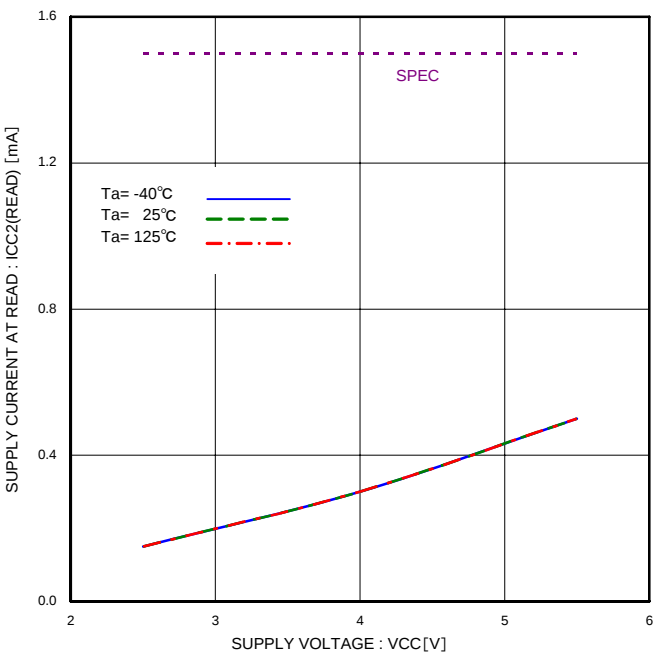
Figure 13. Supply Current at READ Operation vs. Supply Voltage (READ, f_{SK}=2.0\text{MHz} )
