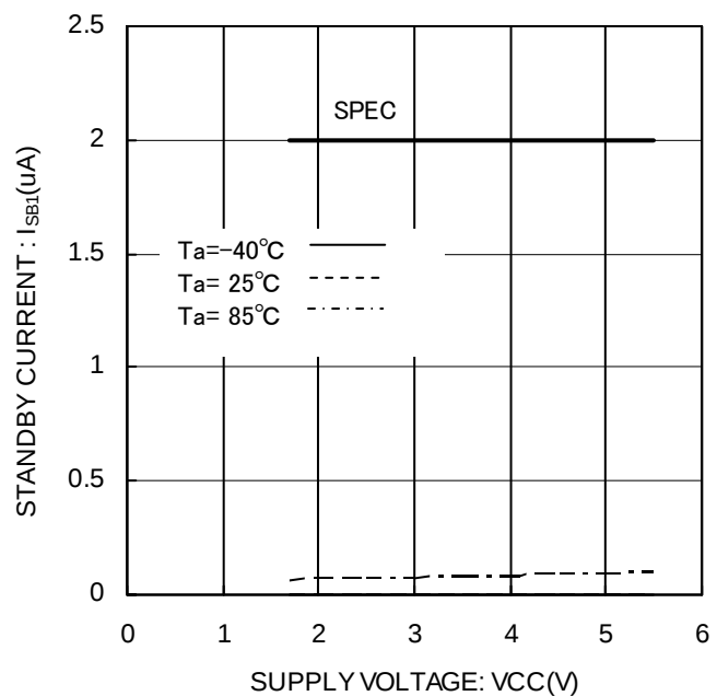
Figure 19. Standby current I_{SBI}(\text{CS}=0\text{V}, \text{ORG}=\text{VCC or OPEN})
