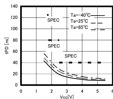
Fig.23 Data output delay time t_{PD}
