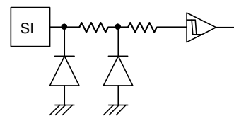
Fig.50 SI input equivalent circuit
