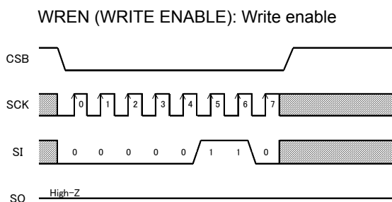
Fig.32 Write enable command
