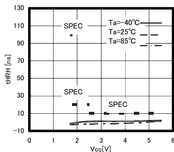
Fig.26 HOLDB release hold time t_{HRH}
