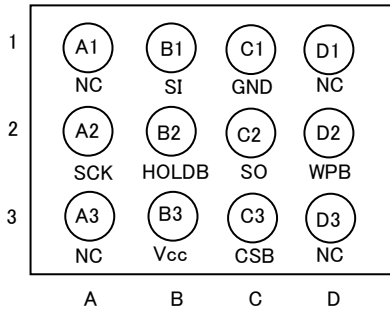
Fig.2 Pin assignment diagram (Bottom View)
