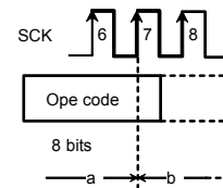
Fig.43 WREN/WRDI cancel valid timing
