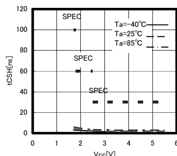
Fig.20 CSB hold time t_{CSH}
