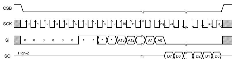
Fig.34 Read command
