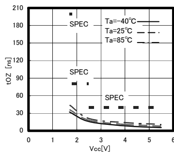
Fig.24 Output disable time t_{OZ}
