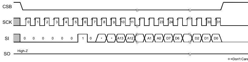
Fig.35 Write command
