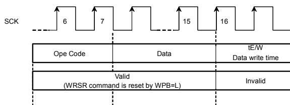
Fig.38 WPB valid timing (At inputting WRSR command)
