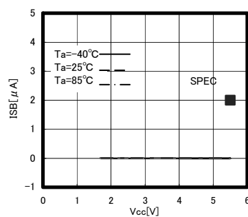
Fig.14 Current Consumption at standby operation I_S
