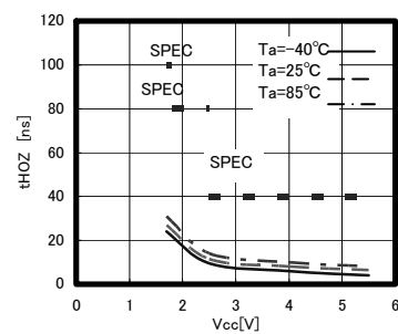
Fig.27 Time from HOLDB to output High-Z t_{HOZ}
