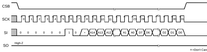
Fig.36 Write command
