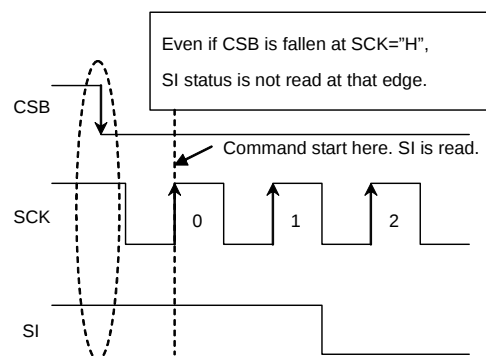
Fig.55 Operating timing
