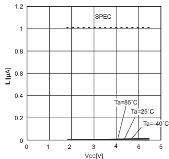
Fig.12 Input leak current I_{LI}(CS,SCK,SI,HOLD)
