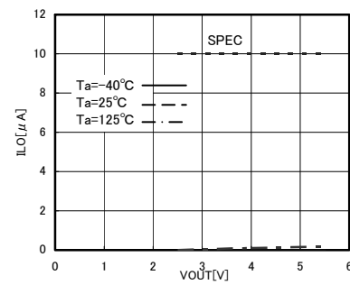
Fig.11 Output leak current I_{LO}(SO)(V_{CC}=5.5V)
