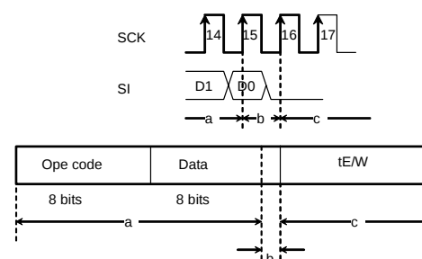
Fig.49 WRSR cancel valid timing
