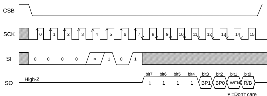
Fig.41 Status register read command (BR25H010/020/040-WC)
