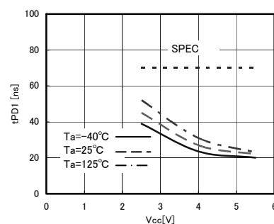
Fig.23 Data output delay time t_{PD1} (CL=100pF)
