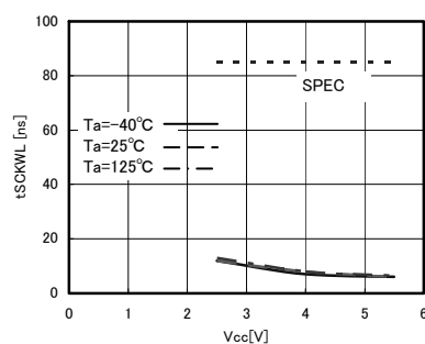
Fig.17 SCK low time t_{SCKWL}
