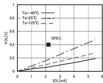
Fig.8 "L" output voltage V_{OL}-I_{OL}(V_{CC}=2.5V)
