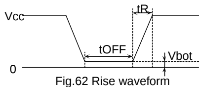
Fig.62 Rise waveform
