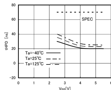
Fig.29 Time from HOLDB to output change t_{HPD}
