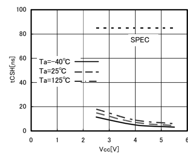
Fig.20 CSB hold time t_{CSH}
