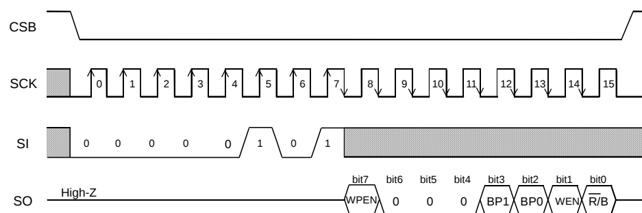
Fig.42 Status register read command (BR25H080/160/320-WC)
