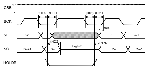
Fig.5 HOLD timing
