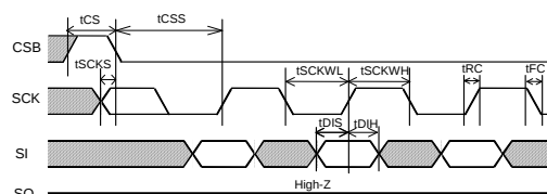
Fig.3 Input timing
