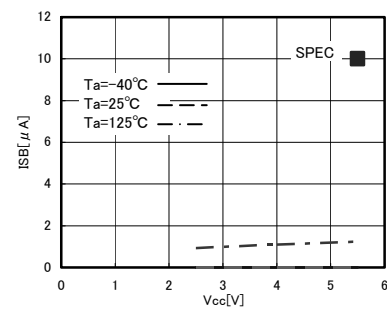
Fig.14 Consumption current at standby operation ISB
