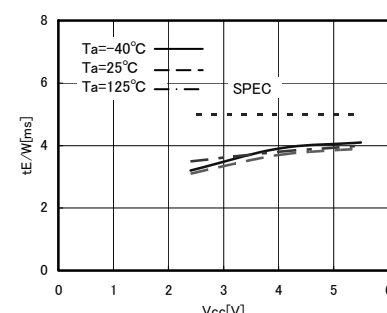
Fig.32 Write cycle time t_{E/W}
