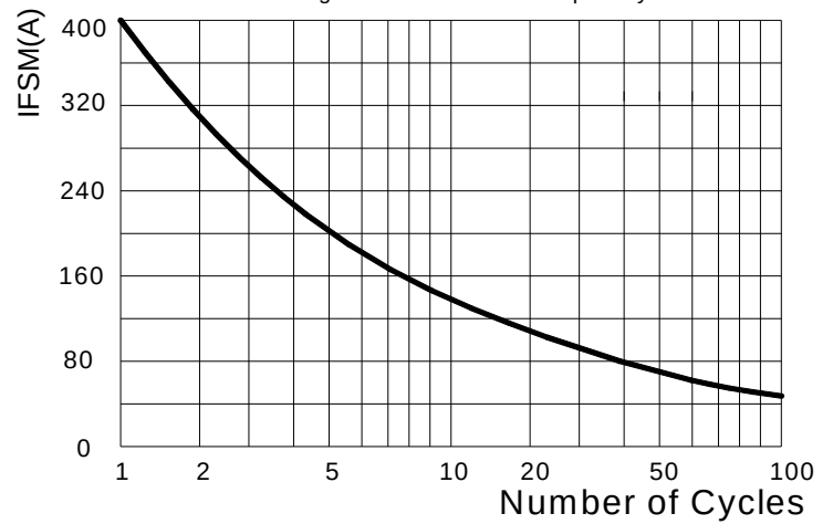
图2: 耐正向浪涌电流曲线 FIG2: Surge Forward Current Capability
