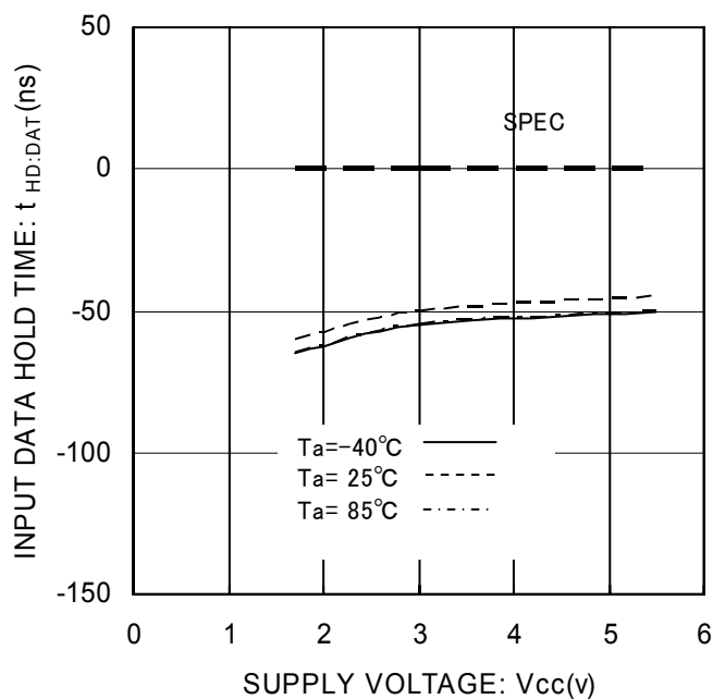
Fig.20 Input Data Hold Time t_{HD} : DAT(LOW)
