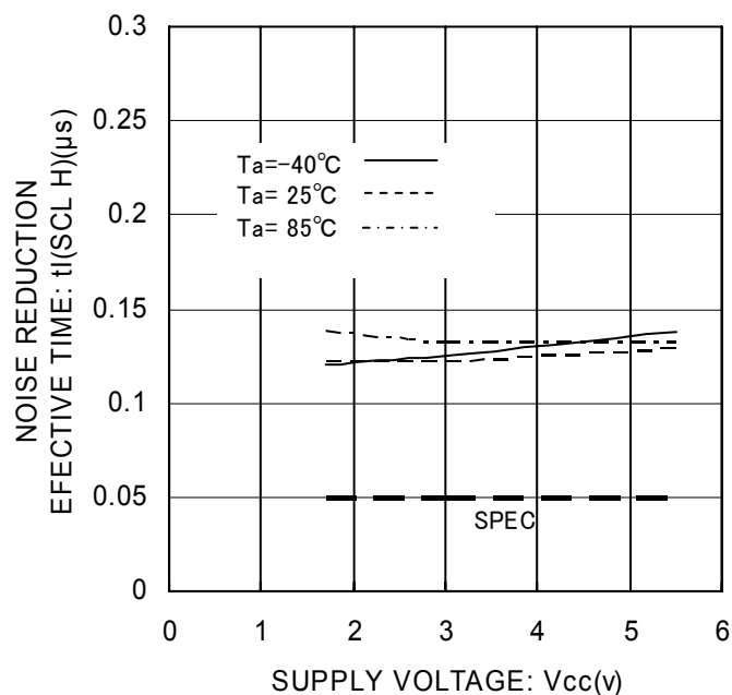
Fig. 28 Noise Spike Width t_i (SCL H)
