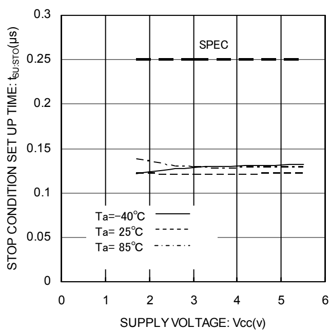
Fig.25 Stop Condition Setup Time t_{SU:sto}
