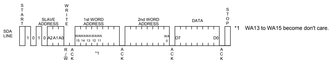
Fig.36 Byte write cycle
