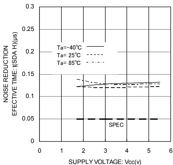
Fig. 30 Noise Spike Width t_i (SDA H)
