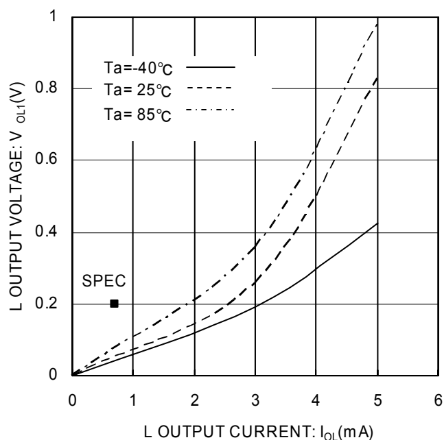
Fig.7 'L' output voltage V_{OL2} ( V_{CC} = 1.7\text{V} )
