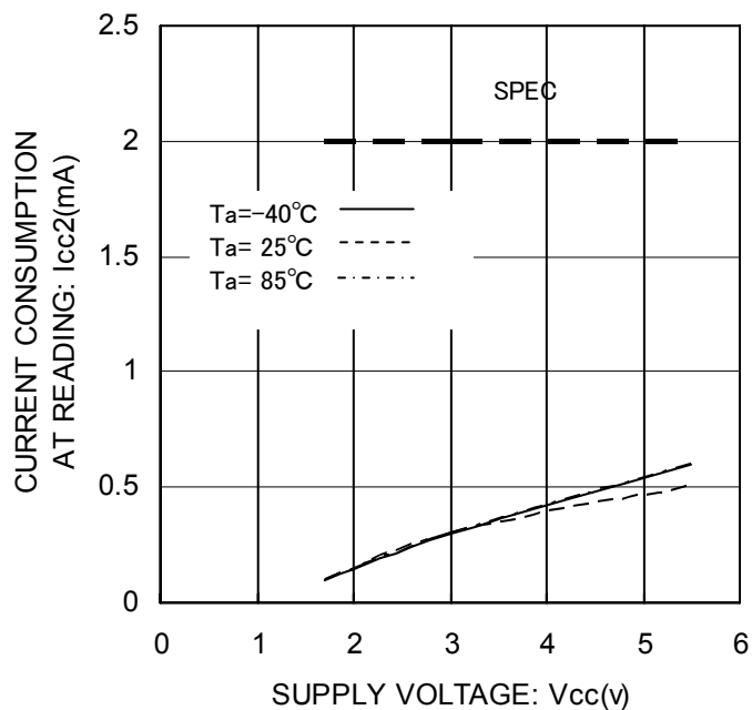
Fig.11 Current consumption at READ operation I_{cc2} ( f_{scl}=1\text{MHz} )
