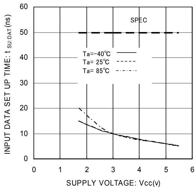
Fig.21 Input Data Setup Time t_{SU} : DAT(HIGH)
