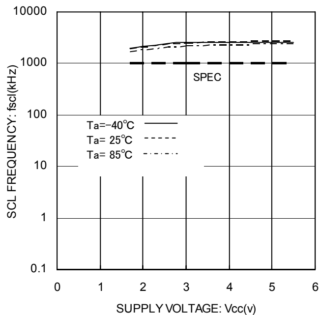
Fig.13 Clock Frequency f_{SCL}
