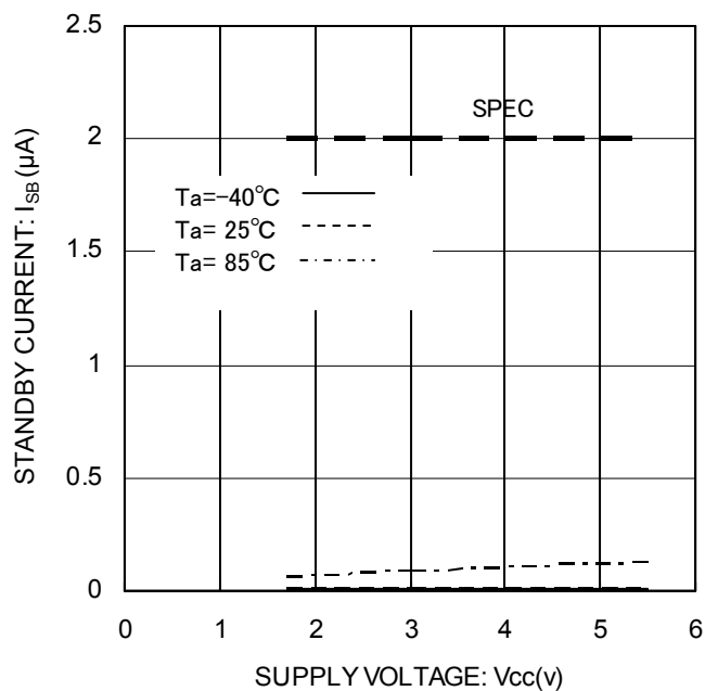
Fig.12 Standby operation I_{SB}
