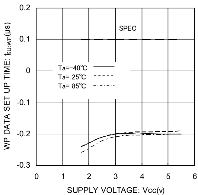
Fig. 33 WP Setup Time t_{SU:WP}
