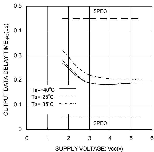
Fig.23 Output Data Delay Time t_{PD0}
