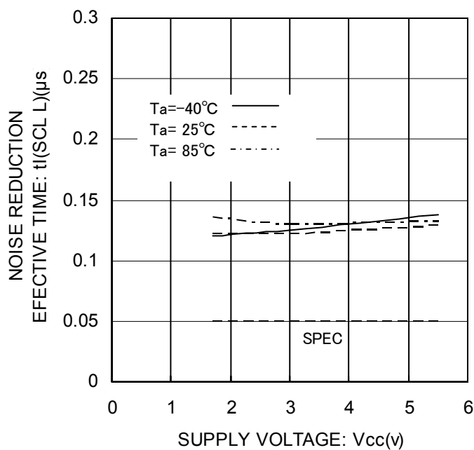
Fig. 29 Noise Spike Width t_i (SCL L)
