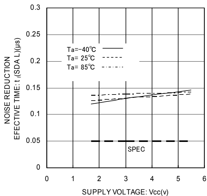
Fig. 31 Noise Spike Width t_i (SDA L)
