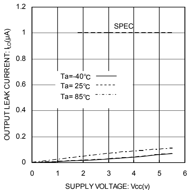
Fig.9 Output leak current I_{LO}(\text{SDA})
