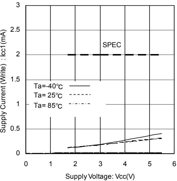
Figure 10. Supply Current (Write) vs Supply Voltage ( f_{SCL}=400kHz )
