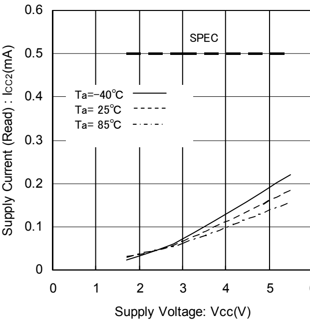
Figure 11. Supply Current (Read) vs Supply Voltage ( f_{SCL}=400kHz )
