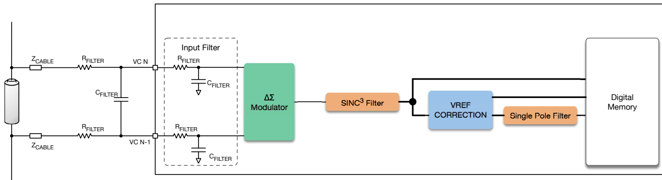
Figure 4. Battery Voltage Signal Chain
