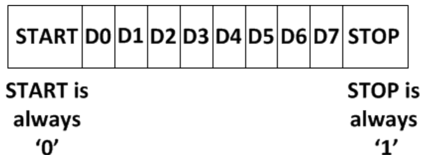
Figure 22. UART Protocol
