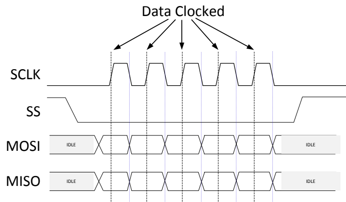
Figure 36. CPOL=0, CPHA=0 Diagram
