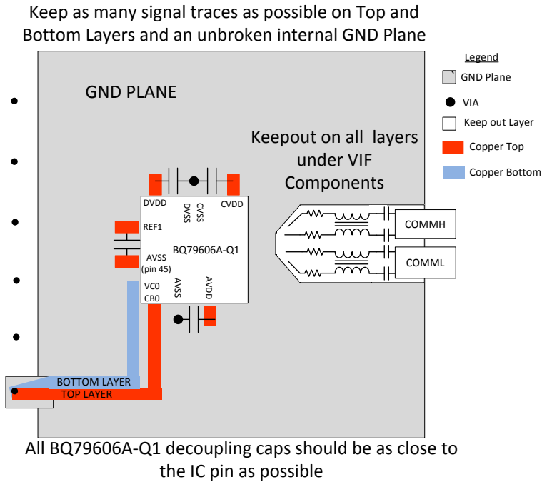
Figure 68. Layout Example
